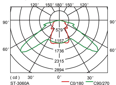
TYPE III DISTRIBUTION
